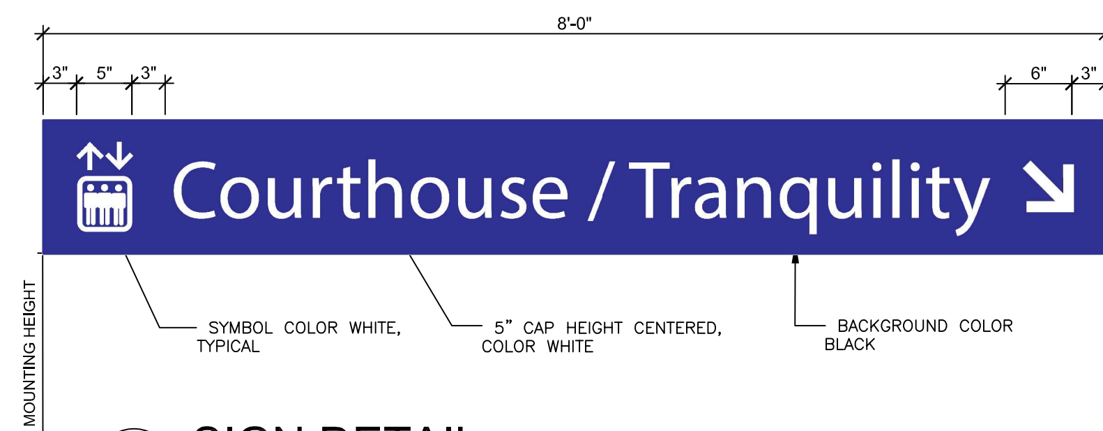
3 SIGN DETAIL
