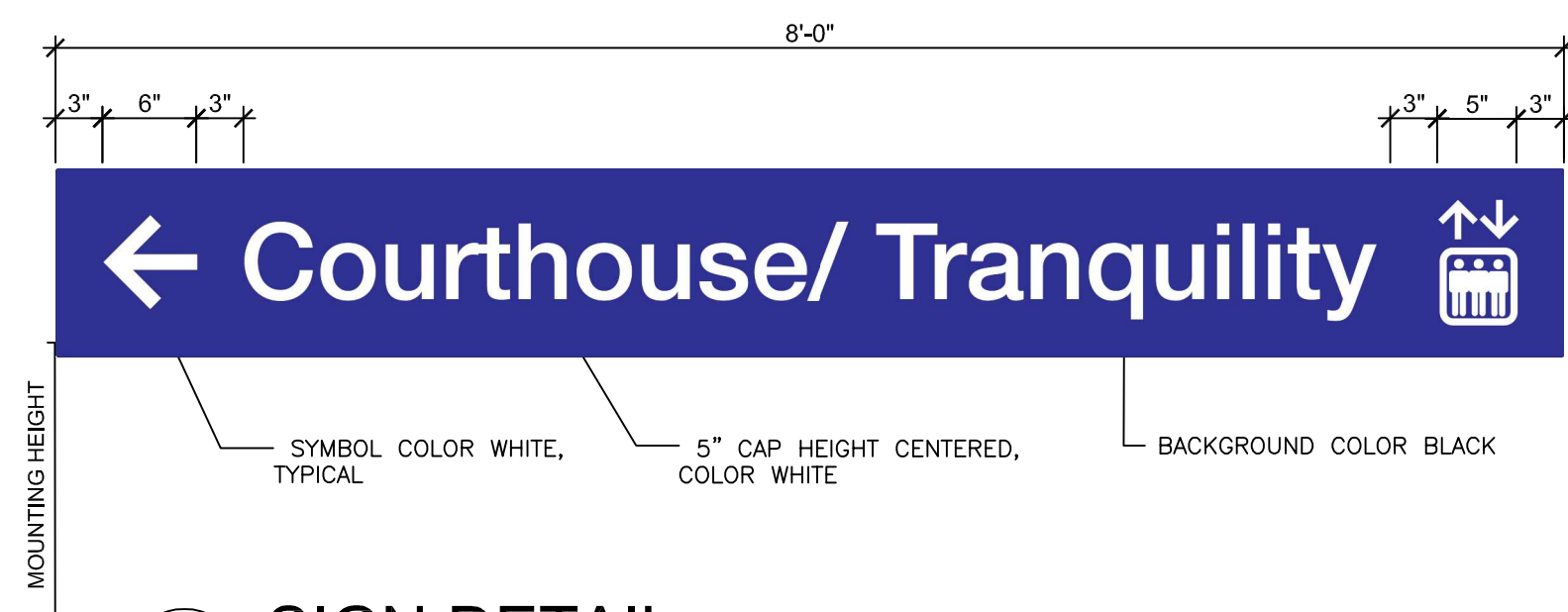
2 SIGN DETAIL
